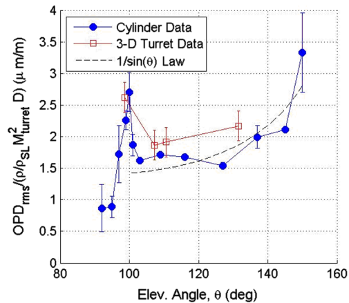
Fig. 7 \text{OPD}_{\text{rms}} as a function of \rho M^2 for selected elevation angles (left). Normalized \text{OPD}_{\text{rms}} as a function of elevation angle (right). Normalized \text{OPD}_{\text{rms}} from a 3-D turret with a flat window [7] is also shown for comparison.
