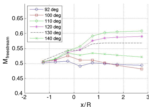
Fig. 3 Mach number distribution along the test section at different elevation angles. Incoming Mach number is 0.4.
