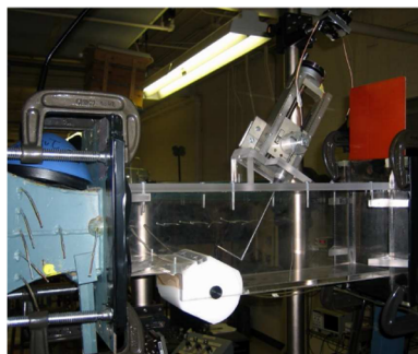
Fig. 9 Malley probe and hot-wire setup for the 120 deg elevation angle (left) and schematic of general hot-wire/Malley probe setup (right).
