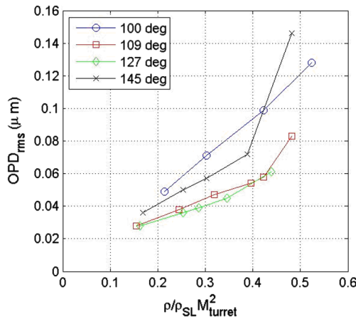
Fig. 7 \text{OPD}_{\text{rms}} as a function of \rho M^2 for selected elevation angles (left). Normalized \text{OPD}_{\text{rms}} as a function of elevation angle (right). Normalized \text{OPD}_{\text{rms}} from a 3-D turret with a flat window [7] is also shown for comparison.
